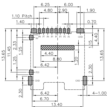
RECOMMEND PCB LAYOUT TOP VIEW TOLERANCE: ±0.05
